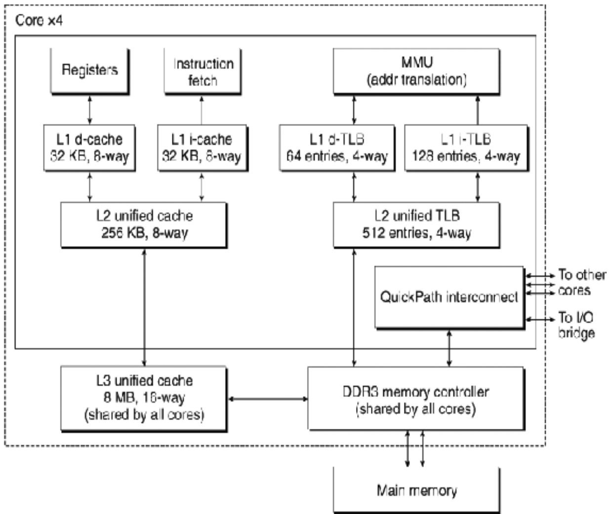
Figure 9.21 The Core i7 memory system.
