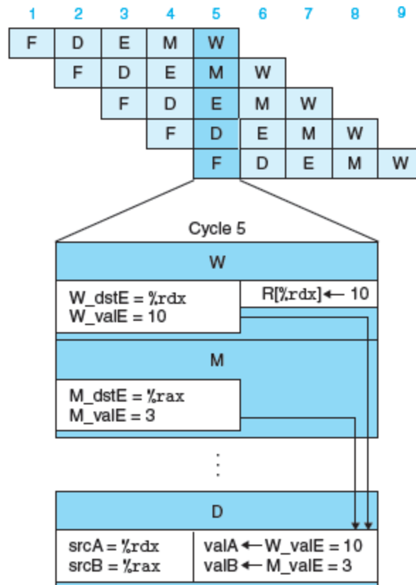
Figure 4.50 Pipelined execution of prog3 using forwarding.
