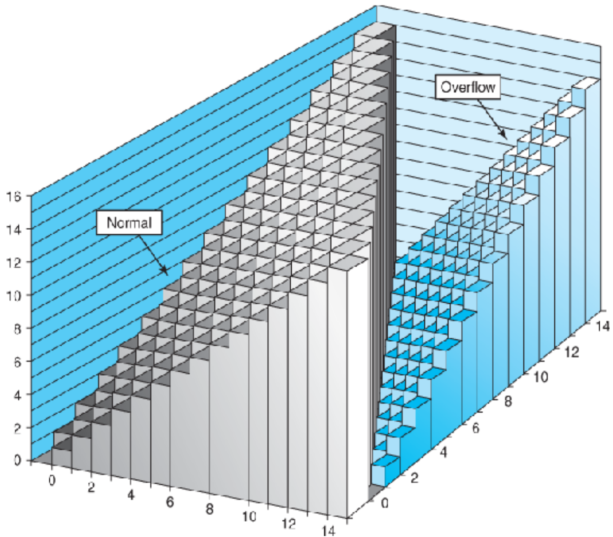
Figure 2.23 Unsigned addition.
