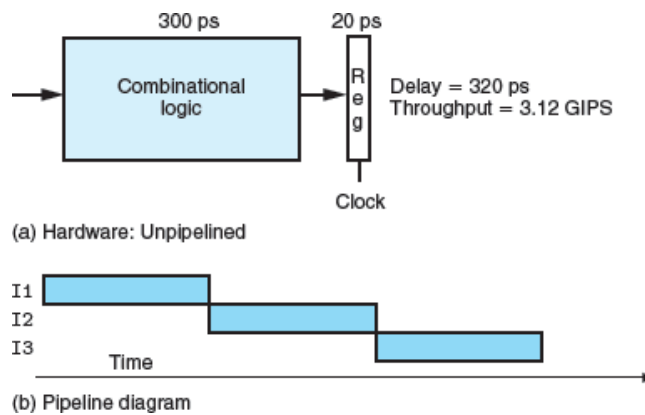
Figure 4.32 Unpipelined computation hardware.
