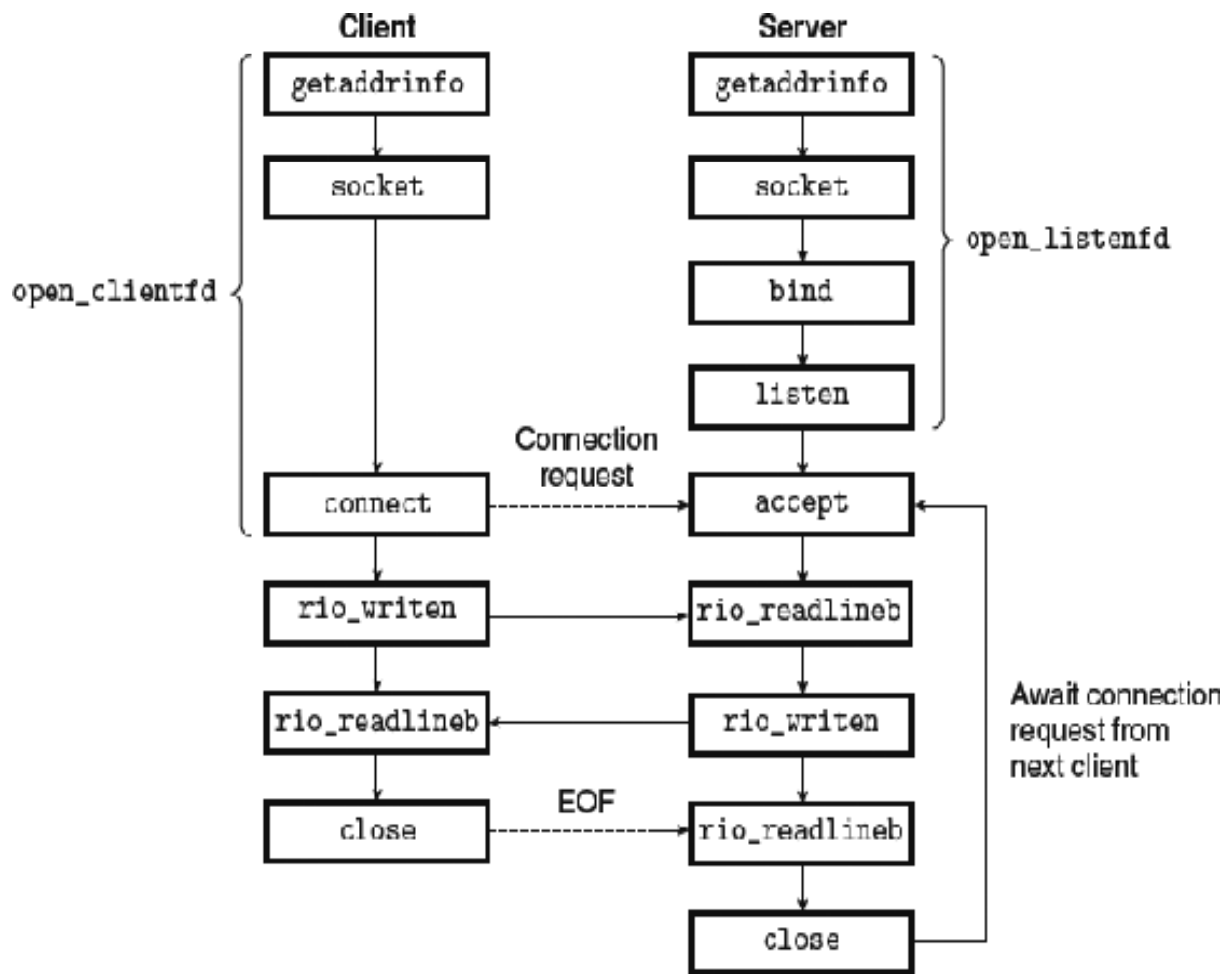
Figure 11.12 Overview of network applications based on the sockets interface.
