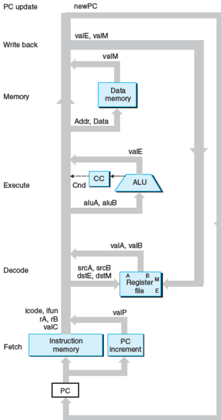
Figure 4.22 Abstract view of SEQ, a sequential implementation.
