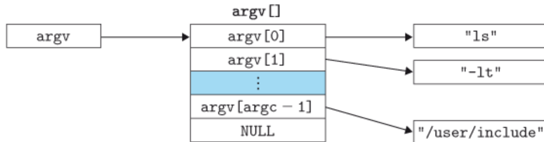
Figure 8.20 Organization of an argument list.
