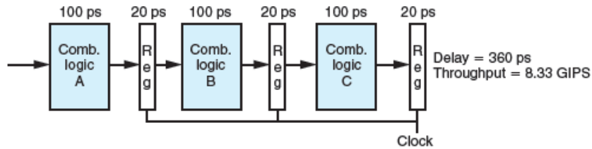
(a) Hardware: Three-stage pipeline
