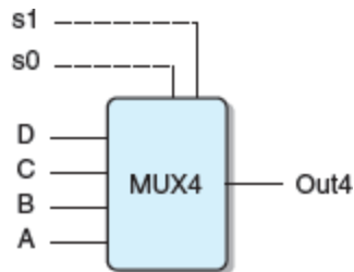
Figure 4.14 Four-way multiplexor.
