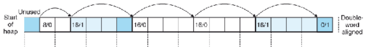
Figure 9.38 An example of false fragmentation.
