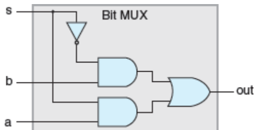
Figure 4.11 Single-bit multiplexor circuit.
