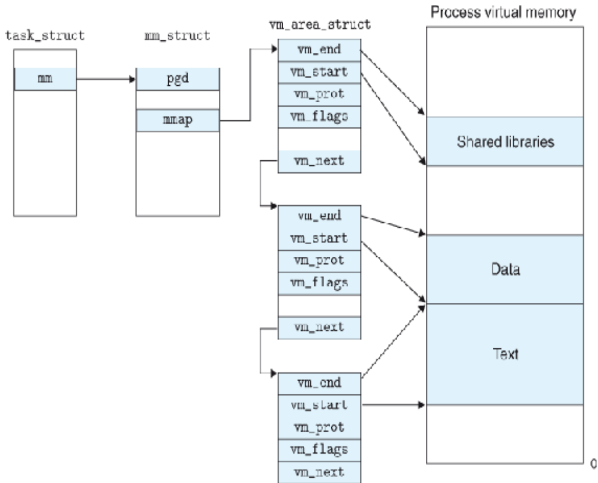
Figure 9.27 How Linux organizes virtual memory.
