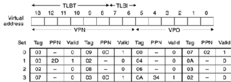
(a) TLB: 4 sets, 16 entres, 4-way set associative
