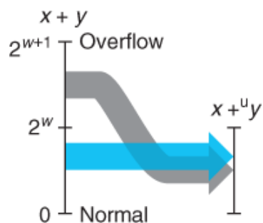
Figure 2.22 Relation between integer addition and unsigned addition.
