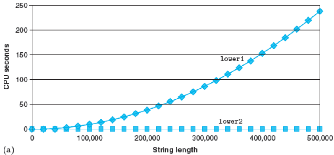
Figure 5.8 Comparative performance of lowercase conversion routines.
