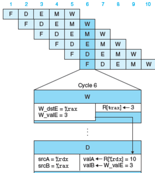
Figure 4.49 Pipelined execution of prog2 using forwarding. In cycle 6, the decode-stage logic detects the presence of a pending write to register %rax in the write-back stage. It uses this value for source operand valB rather than the value read from the register file.
