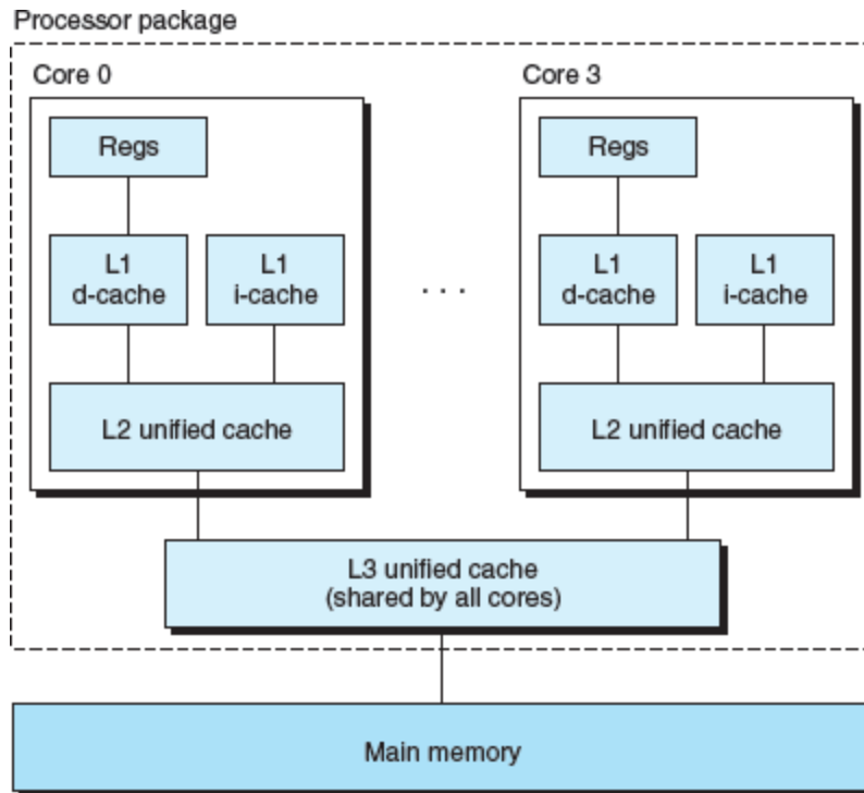
Figure 6.38 Intel Core i7 cache hierarchy.
