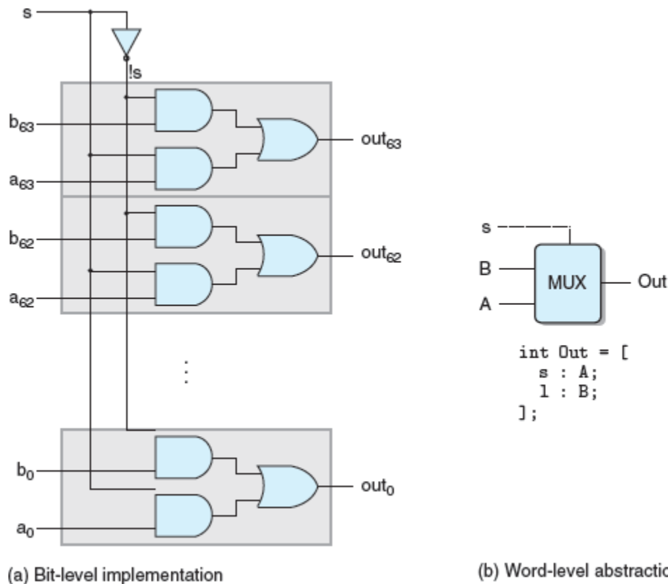
Figure 4.13 Word-level multiplexor circuit.
