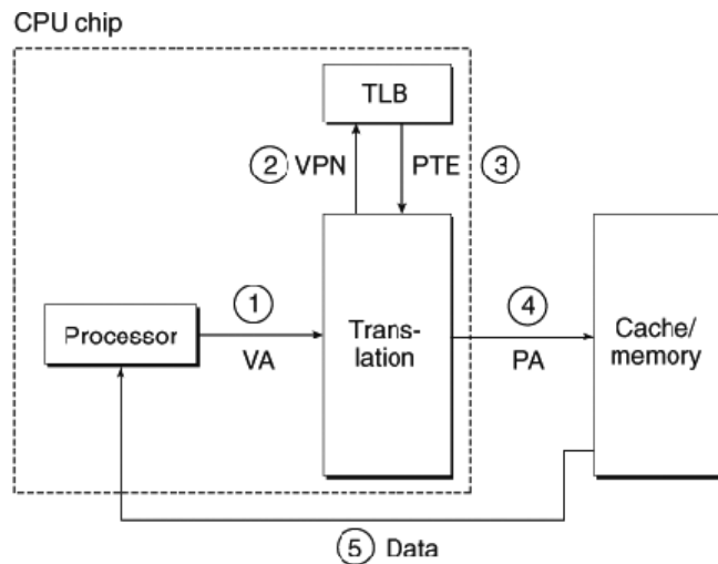
(a) TLB hit
