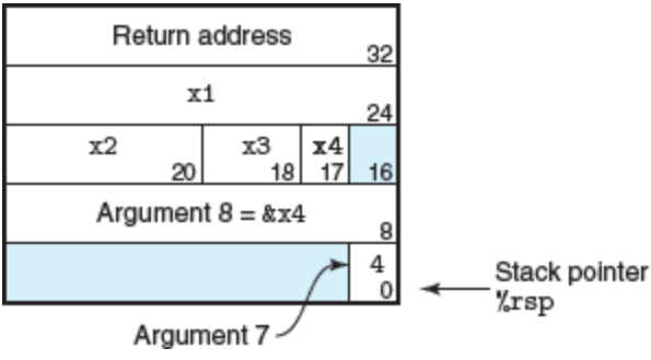
Figure 3.33 Stack frame for function call_proc .
