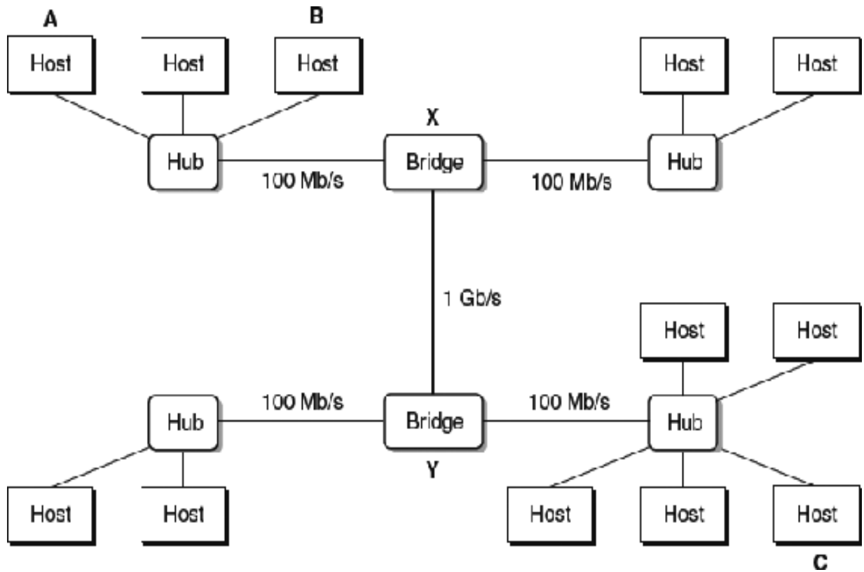
Figure 11.4 Bridged Ethernet segments.
