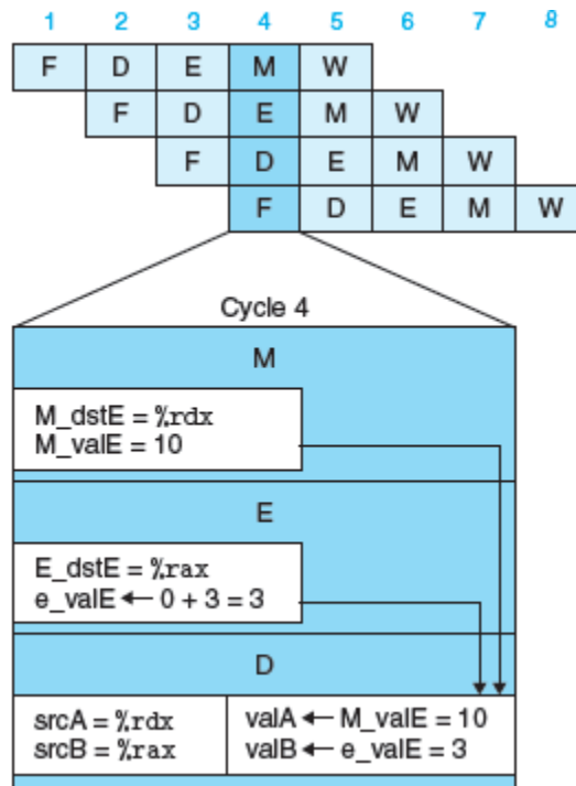
Figure 4.51 Pipelined execution of prog4 using forwarding.
