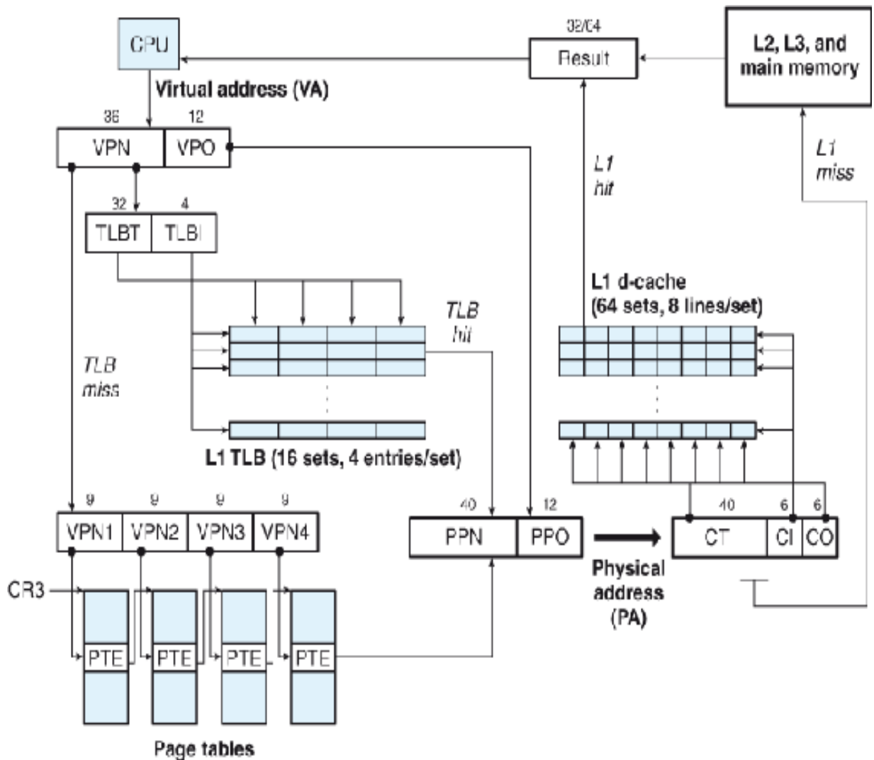
Figure 9.22 Summary of Core i7 address translation.
