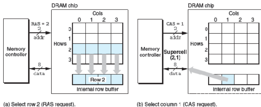
Figure 6.4 Reading the contents of a DRAM supercell.
