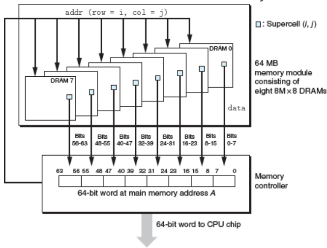
Figure 6.5 Reading the contents of a memory module.
