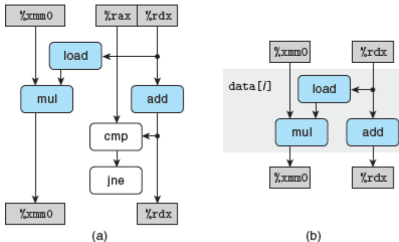
Figure 5.14 Abstracting combine4 operations as a data-flow graph.
