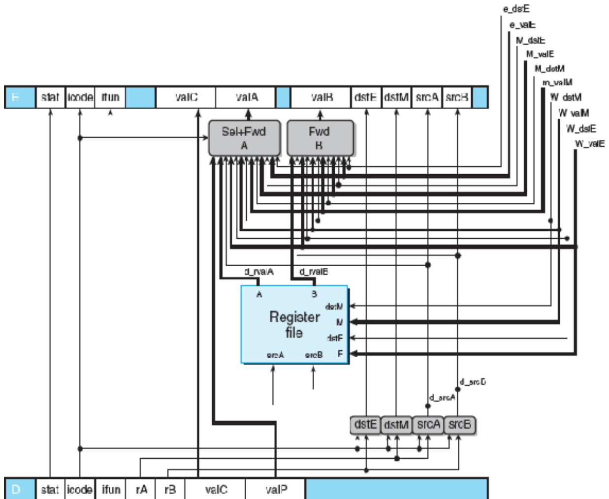
Figure 4.58 PIPE decode and write-back stage logic.
