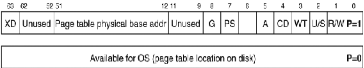
Figure 9.23 Format of level 1, level 2, and level 3 page table entries.
