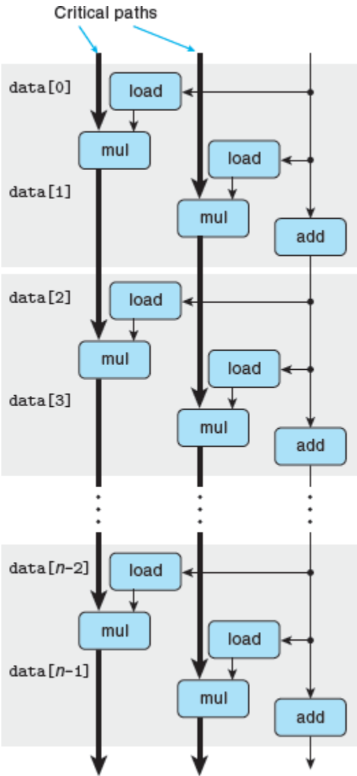
Figure 5.24 Data-flow representation of combine6 operating on a vector of length n .
