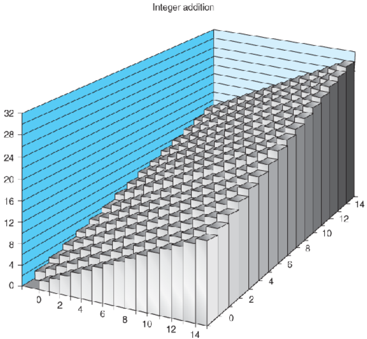
Figure 2.21 Integer addition.
