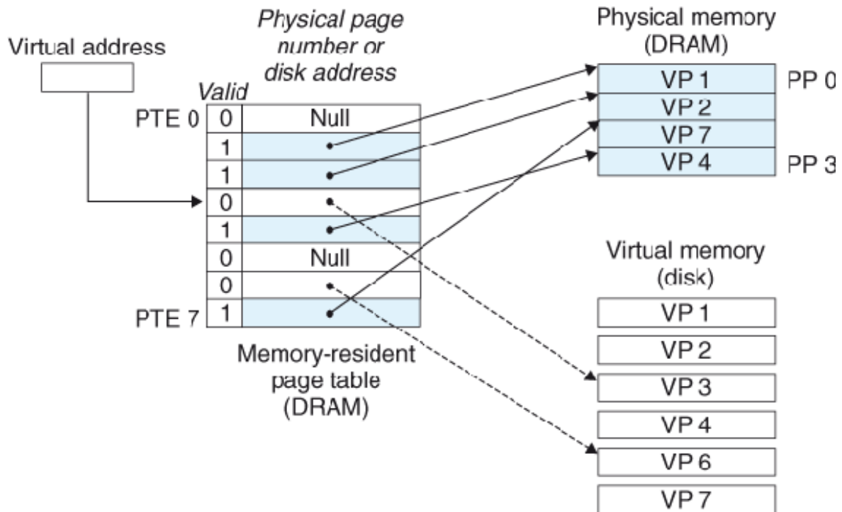
Figure 9.6 VM page fault (before).
