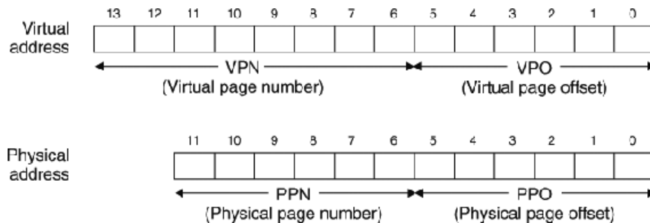
Figure 9.19 Addressing for small memory system.
