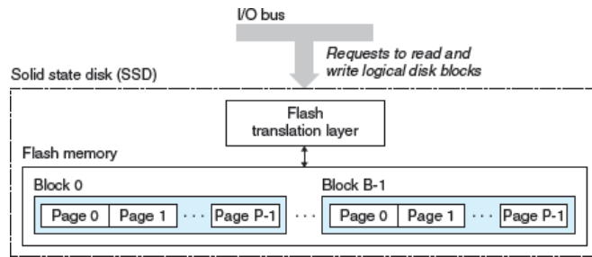
Figure 6.13 Solid state disk (SSD).
