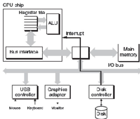
Figure 6.12 Reading a disk sector.
