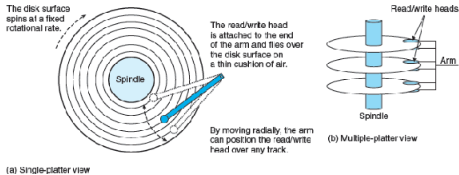
Figure 6.10 Disk dynamics.
