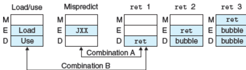
Figure 4.67 Pipeline states for special control conditions.
