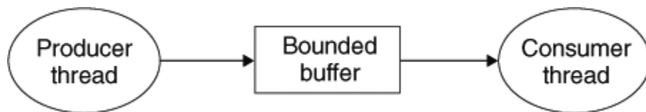
Figure 12.23 Producer-consumer problem.
