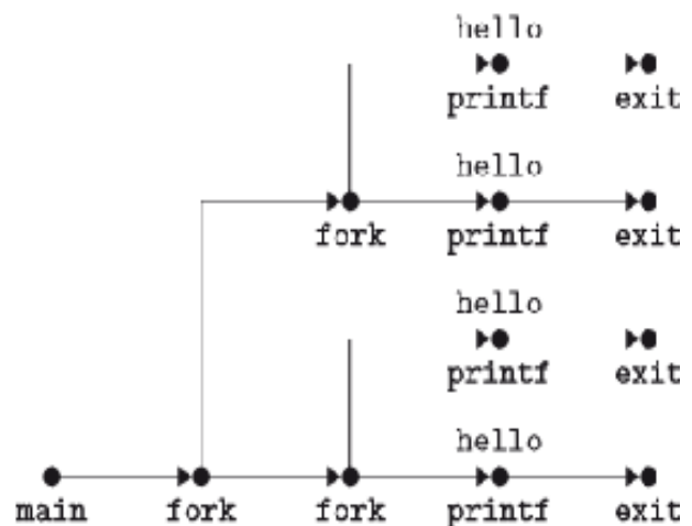
Figure 8.17 Process graph for a nested fork .
