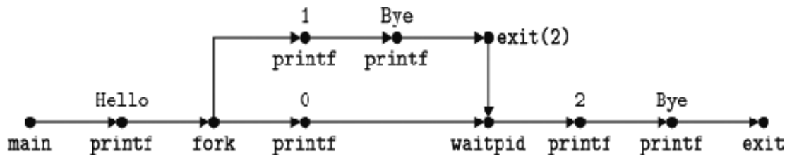
Figure 8.49 Process graph for Practice Problem 8.4 .
