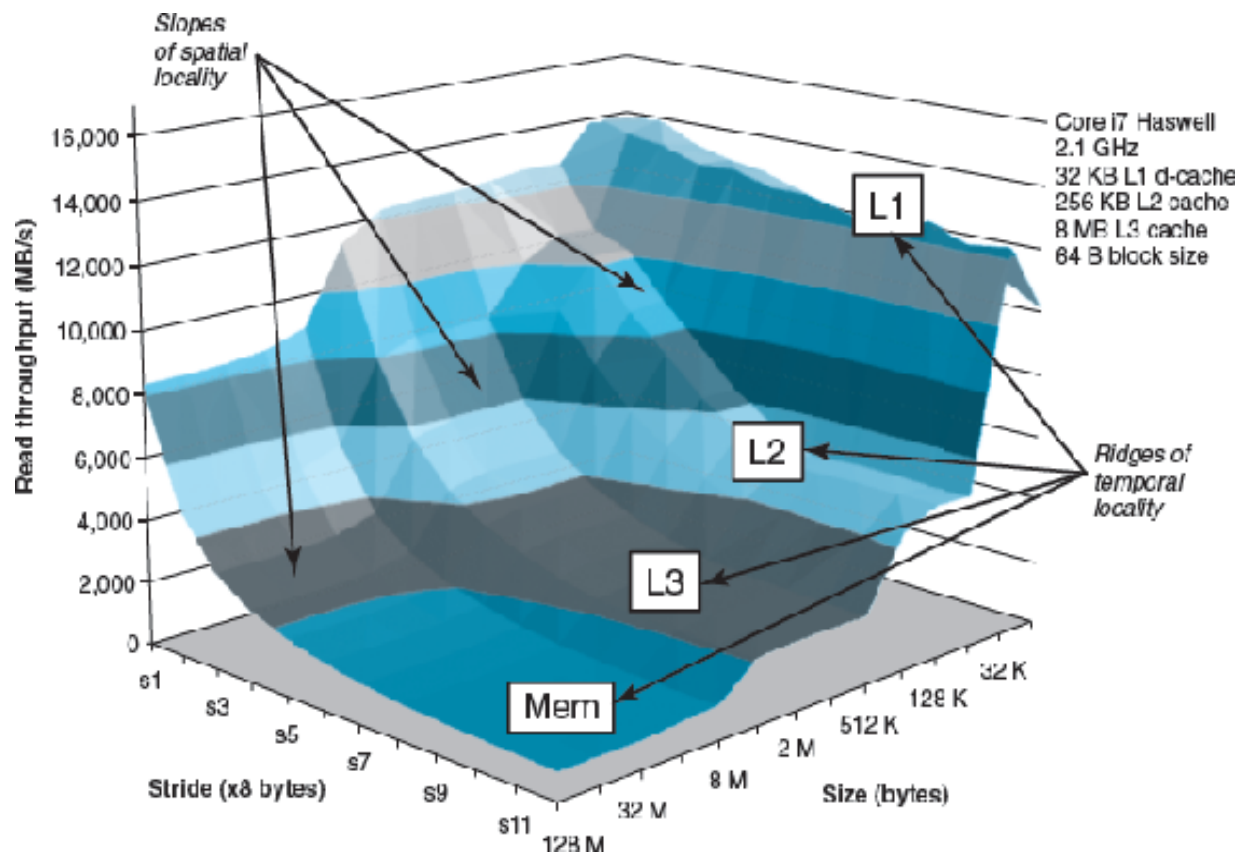
Figure 6.41 A memory mountain.
