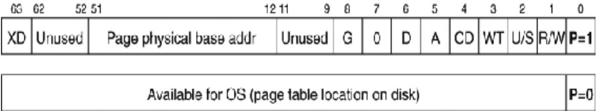
Figure 9.24 Format of level 4 page table entries.
