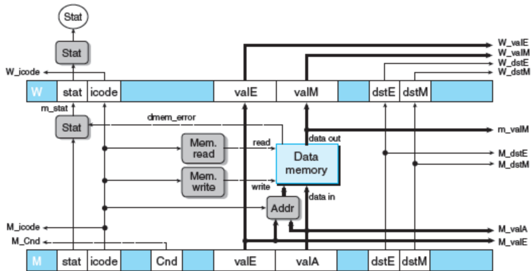
Figure 4.61 PIPE memory stage logic.
