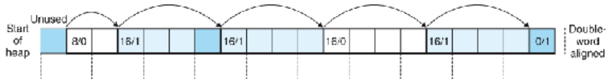
Figure 9.37 Splitting a free block to satisfy a three-word allocation request.
