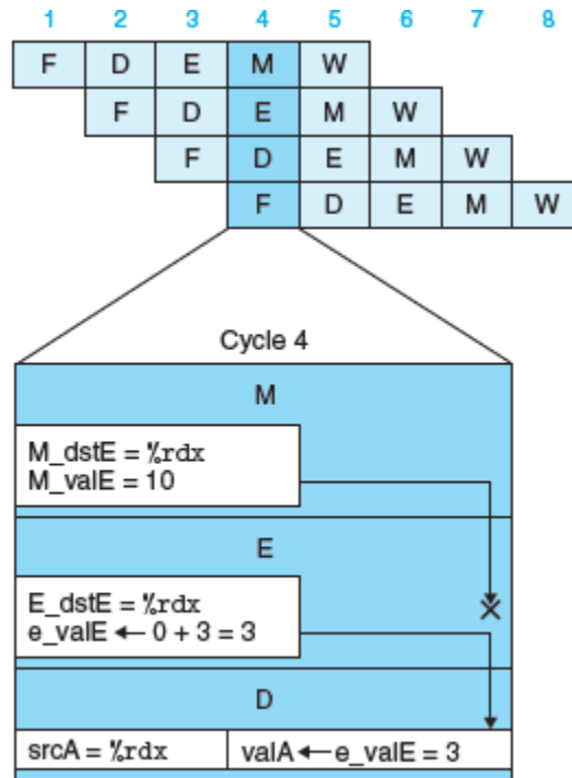
Figure 4.59 Demonstration of forwarding priority.
