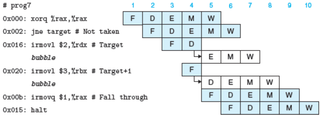
Figure 4.56 Processing mispredicted branch instructions.
