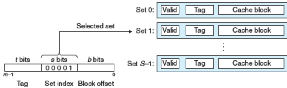
Figure 6.28 Set selection in a direct-mapped cache.
