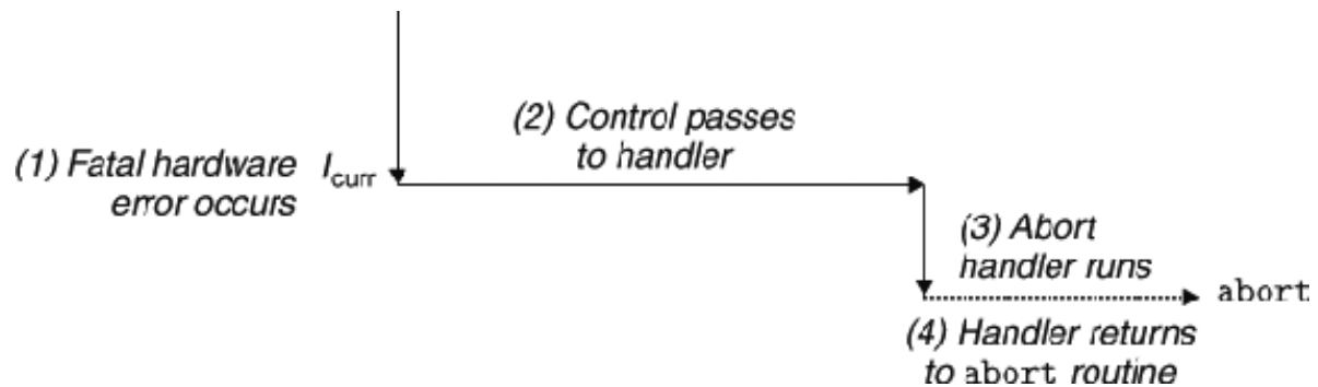
Figure 8.8 Abort handling.
