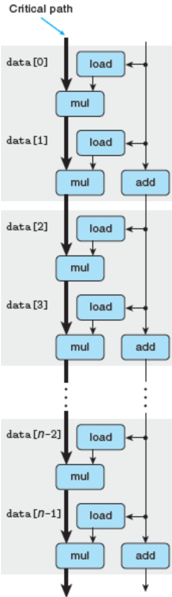
Figure 5.20 Data-flow representation of combine5 operating on a vector of length n .
