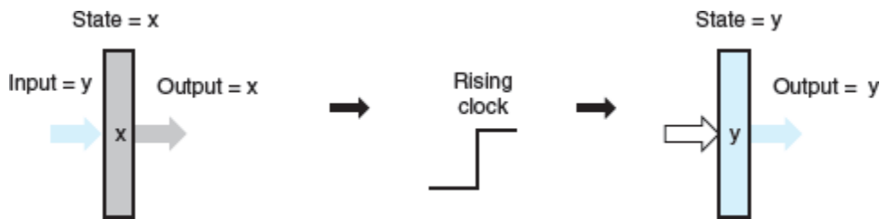
Figure 4.16 Register operation.
