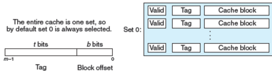
Figure 6.36 Set selection in a fully associative cache.
