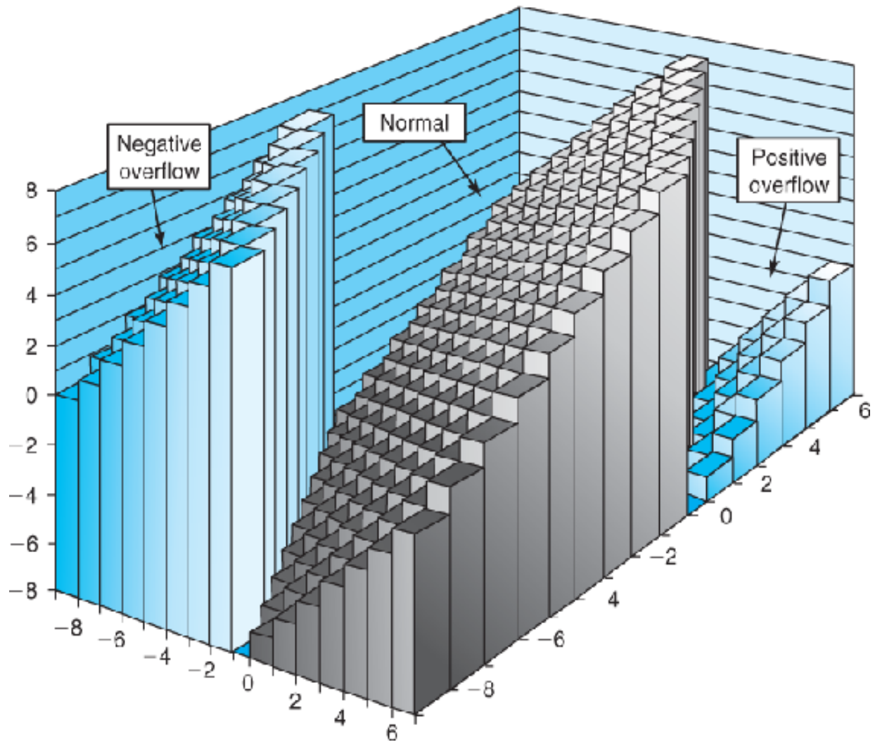
Two's-complement addition (4-bit word)
