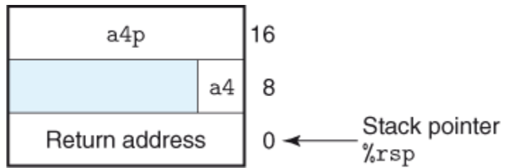
Figure 3.30 Stack frame structure for function proc . Arguments a4 and a4p are passed on the stack.
