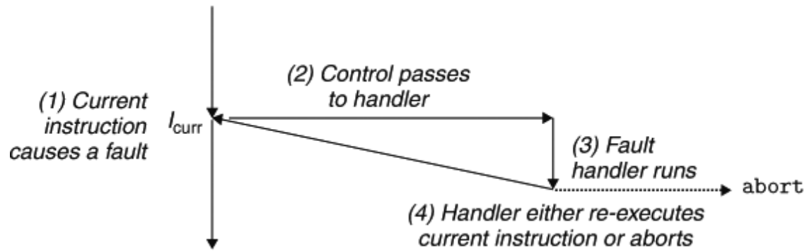
Figure 8.7 Fault handling.
