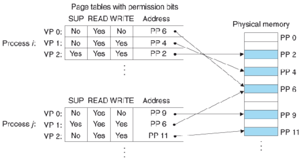
Figure 9.10 Using VM to provide page-level memory protection.
