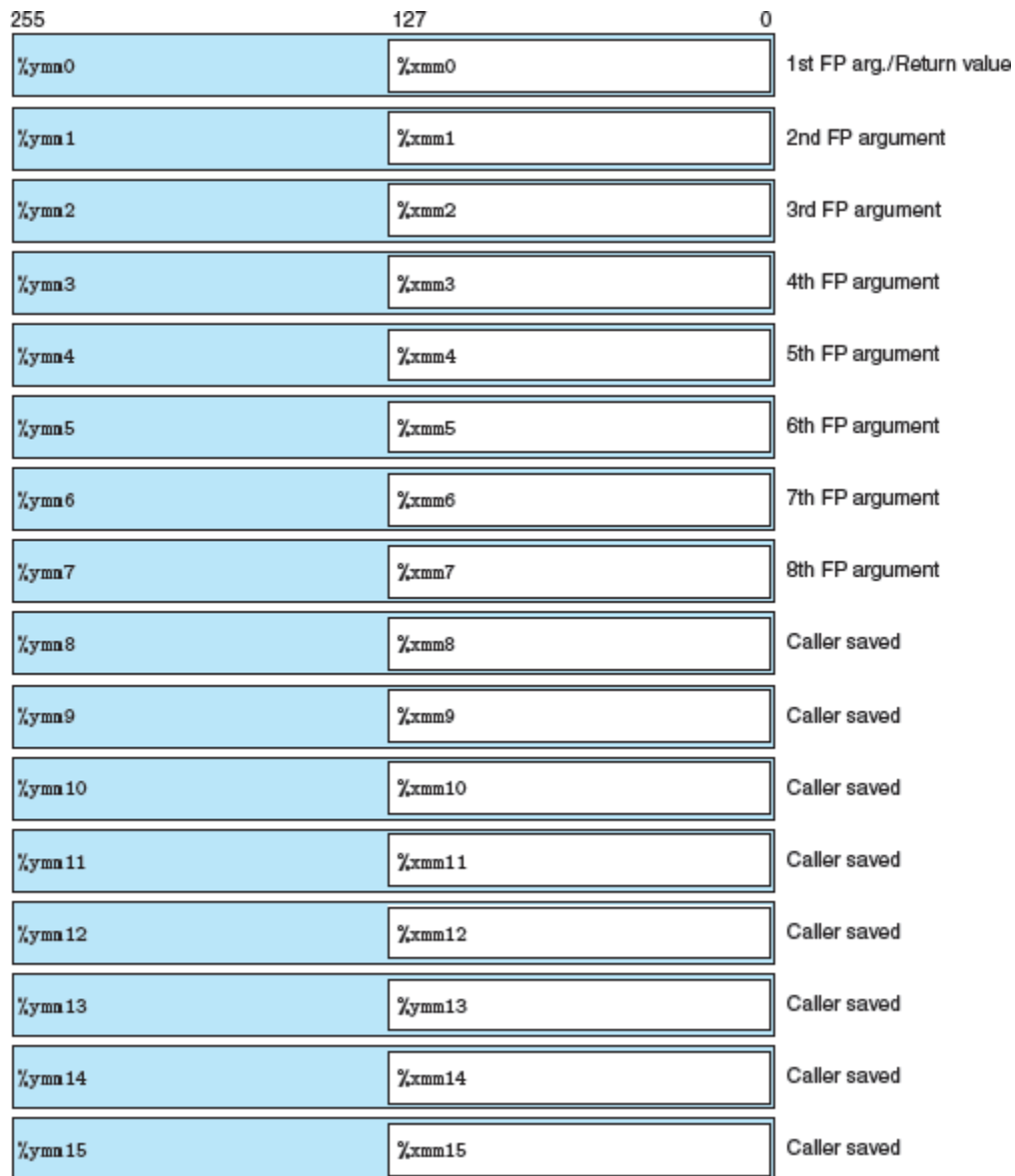
Figure 3.45 Media registers.
