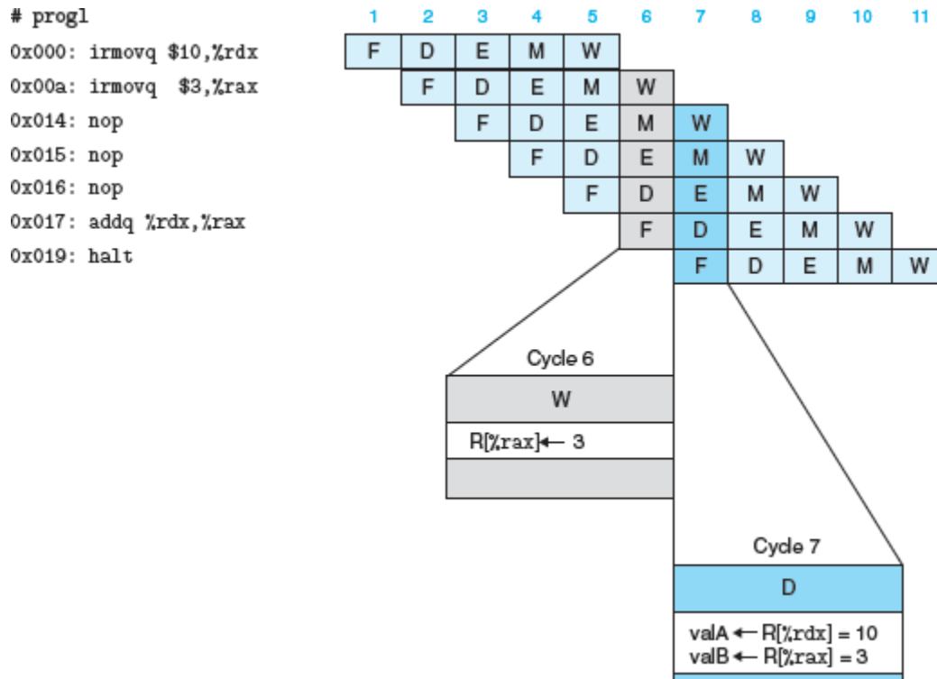
Figure 4.43 Pipelined execution of prog1 without special pipeline control.
