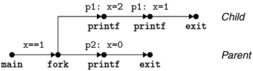
Figure 8.47 Process graph for Practice Problem 8.2 .
