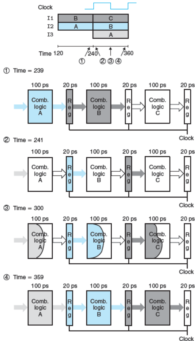
Figure 4.35 One clock cycle of pipeline operation.
