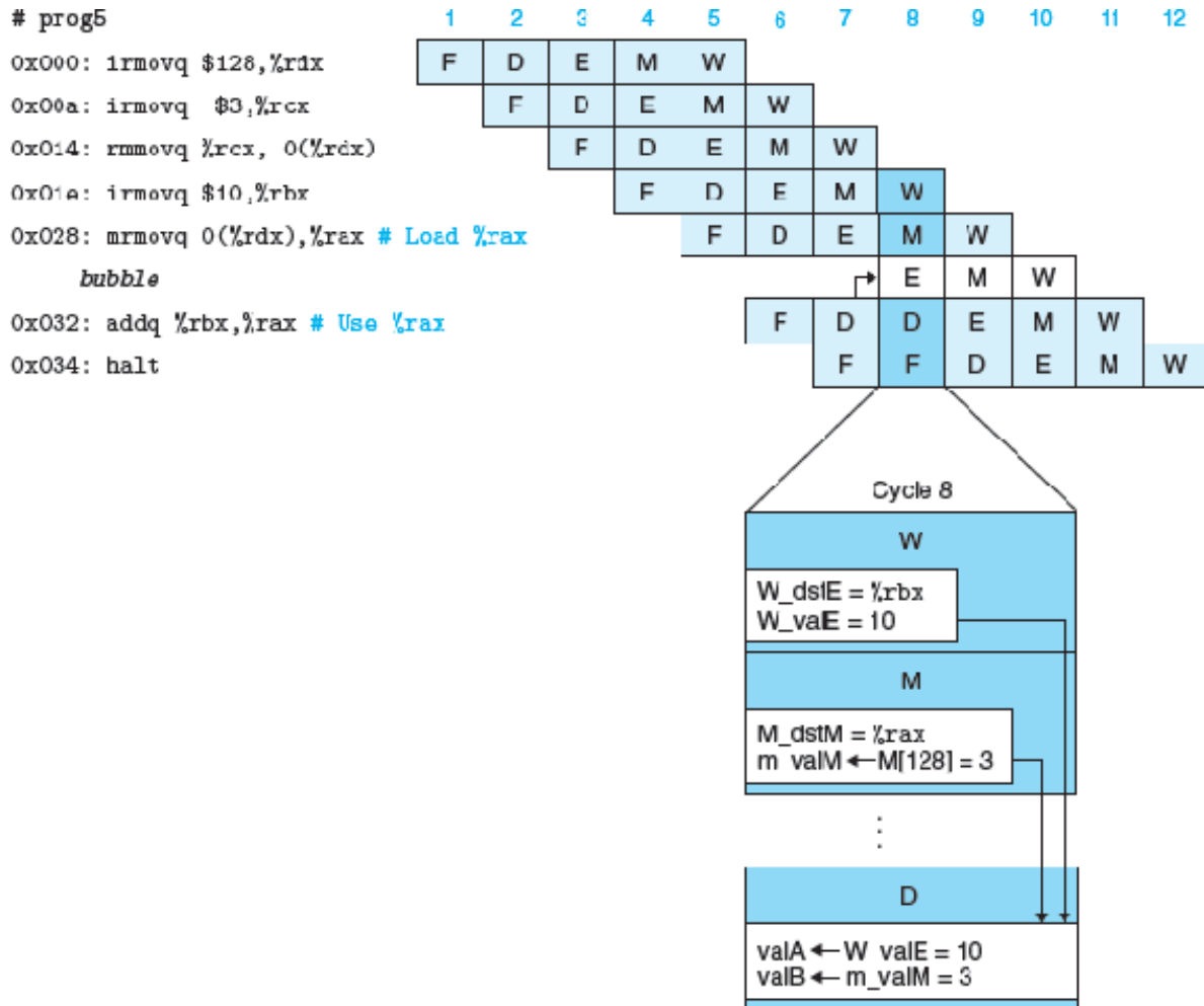
Figure 4.54 Handling a load/use hazard by stalling.
