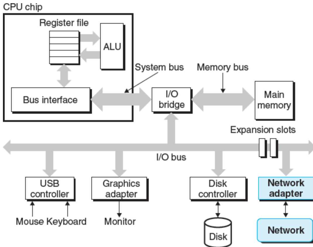
Figure 11.2 Hardware organization of a network host.
