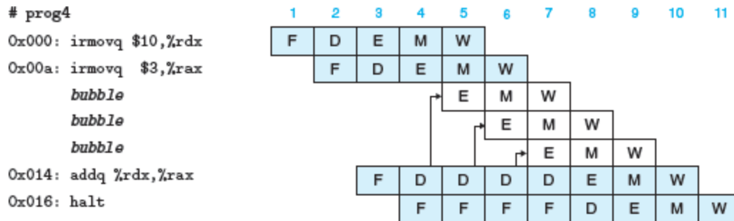
Figure 4.48 Pipelined execution of prog4 using stalls.
