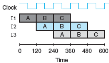
Figure 4.34 Three-stage pipeline timing.
