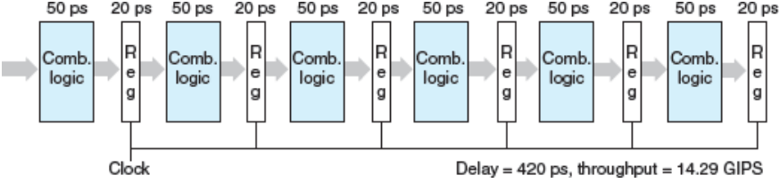
Figure 4.37 Limitations of pipelining due to overhead.
