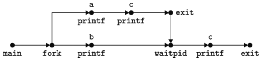
Figure 8.48 Process graph for Practice Problem 8.3 .
