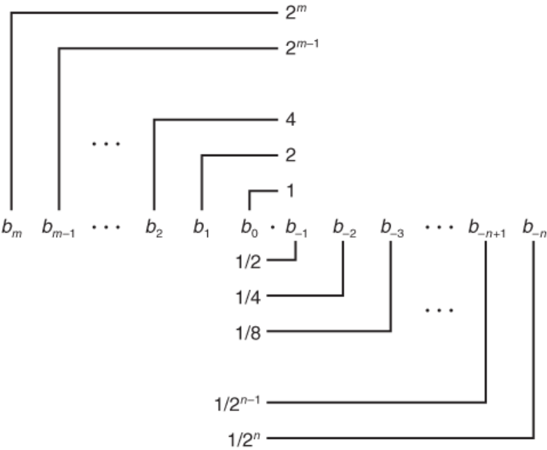
Figure 2.31 Fractional binary representation.
