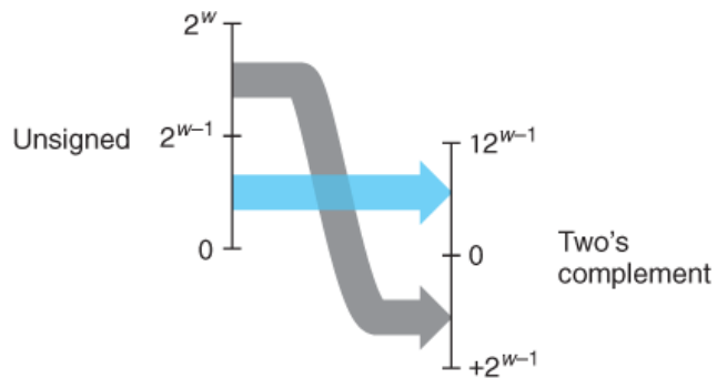
Figure 2.18 Conversion from unsigned to two's complement.
