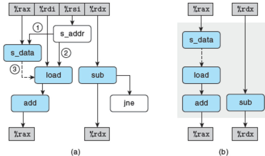
Figure 5.36 Abstracting the operations for write_read .
