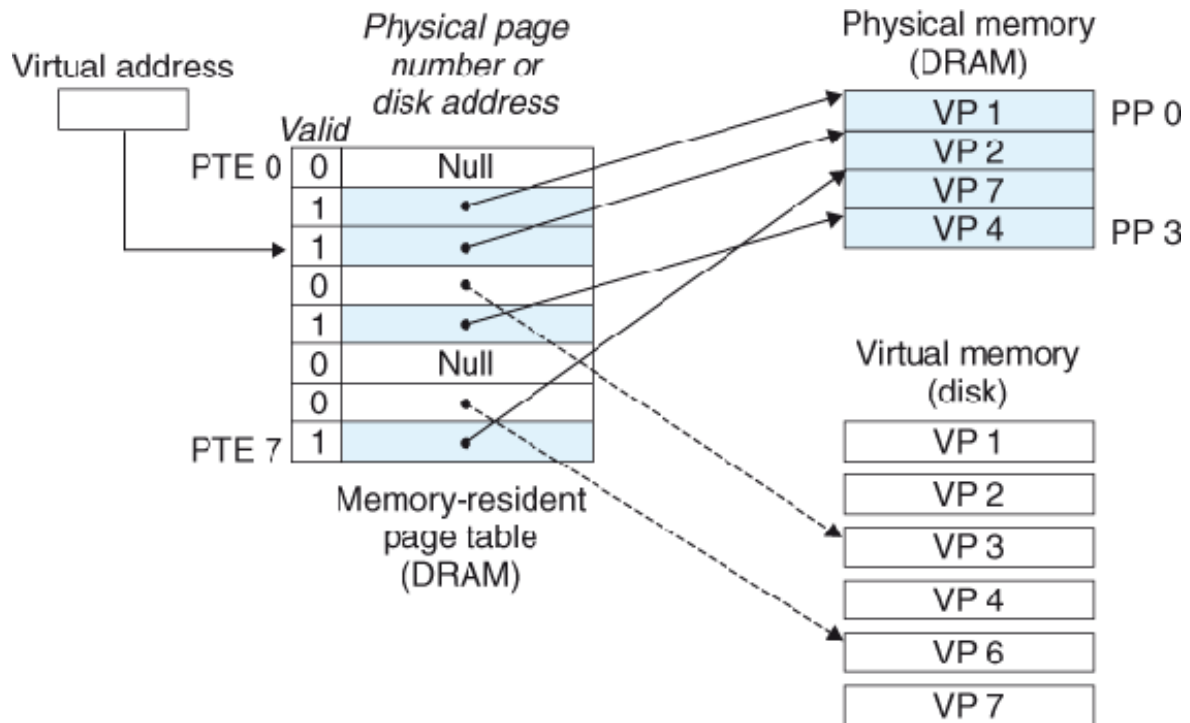
Figure 9.5 VM page hit.
