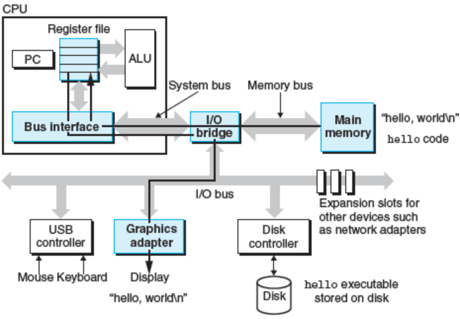
Figure 1.7 Writing the output string from memory to the display.
