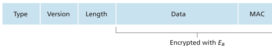
Figure 8.26 ♦ Record format for SSL
